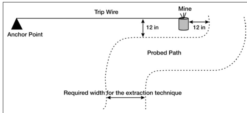
Figure 052-192-1042-6. Marking a Trip Wire
