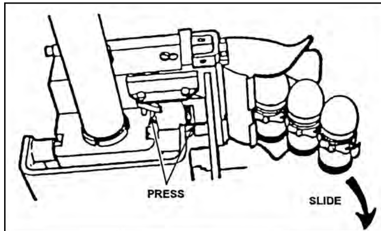
Figure 071-030-0006-2. Removal of Linked Rounds from the Feeder
