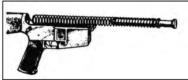
Figure 071-311-2025-24. Placing the spring and buffer
