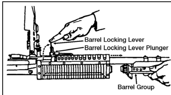
Figure 071-312-3025-11. Barrel locking lever
